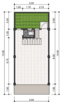
DENAH LANTAI 1
