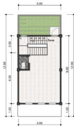
DENAH LANTAI 2
